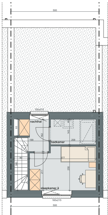
VERDIEPING 2 OPP. ± 26M 2
