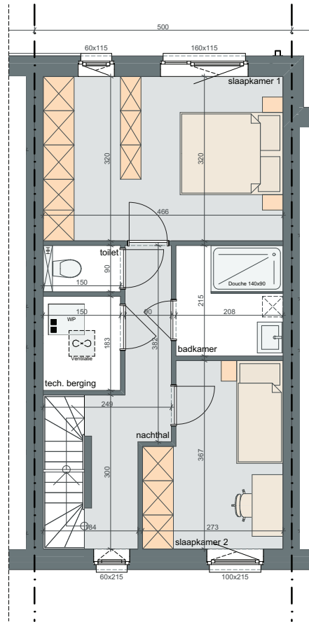
VERDIEPING 1 OPP. ± 50M 2
