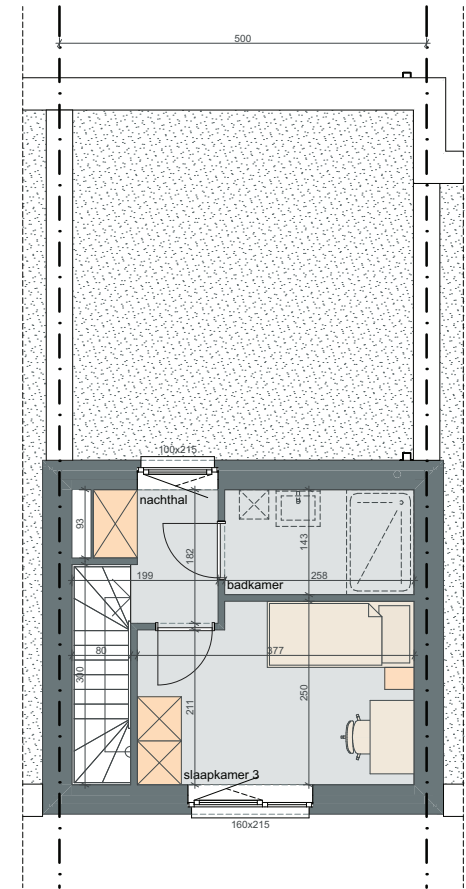
VERDIEPING 2 OPP. ± 26M 2
